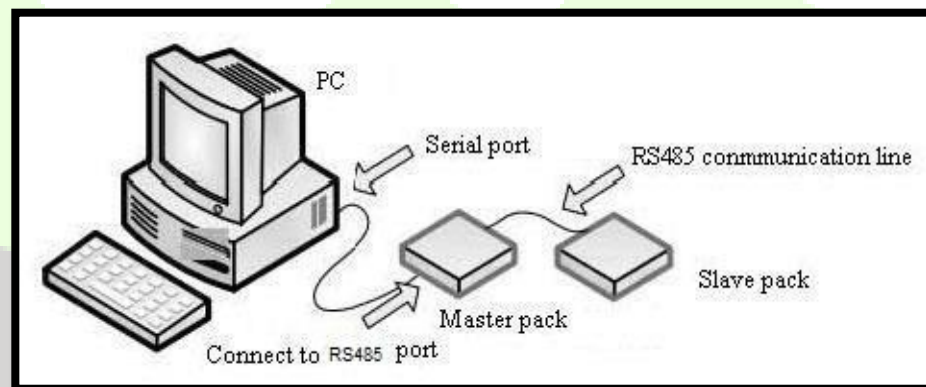
Figure2-4 RS-485 connection schematic diagram
